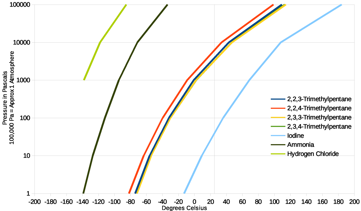
Vapor Pressure of Compounds Associated With Illegal Drugs
