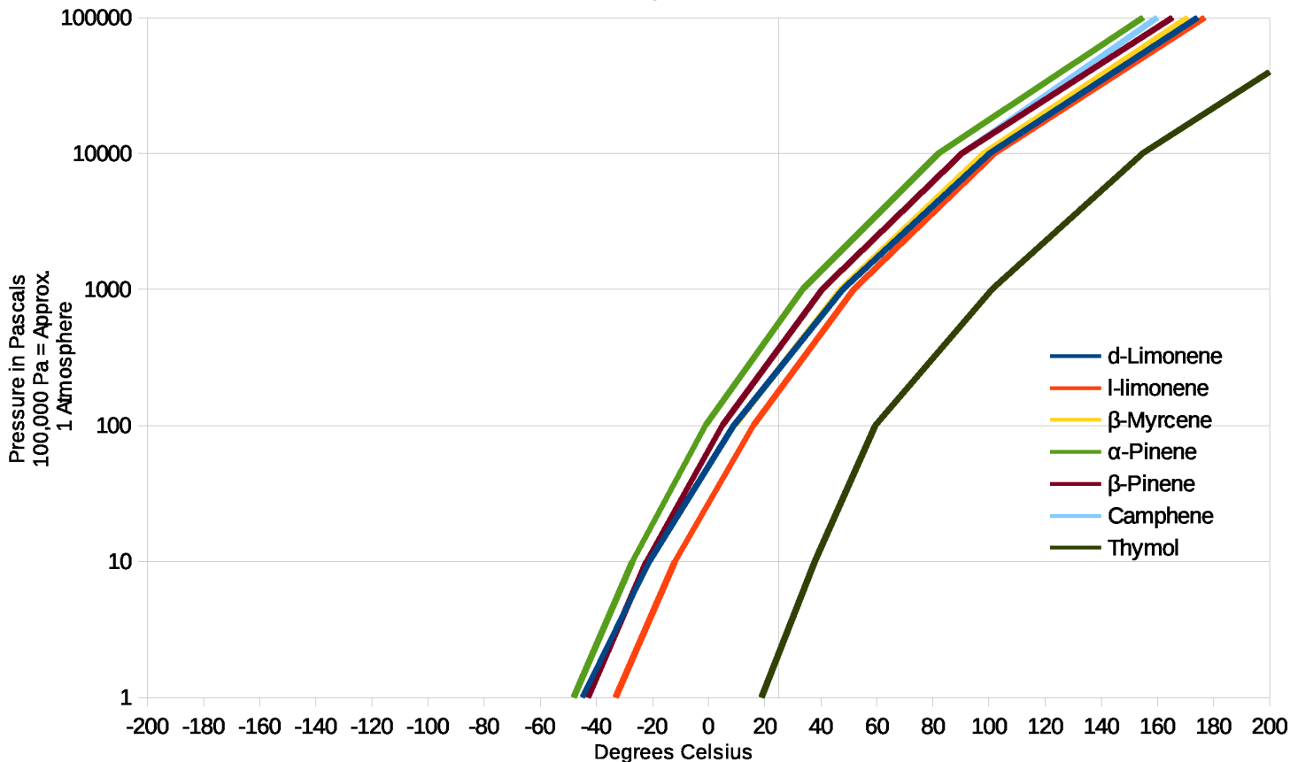
Vapor Pressure of Various Terpenes Associated With C. Sativa
